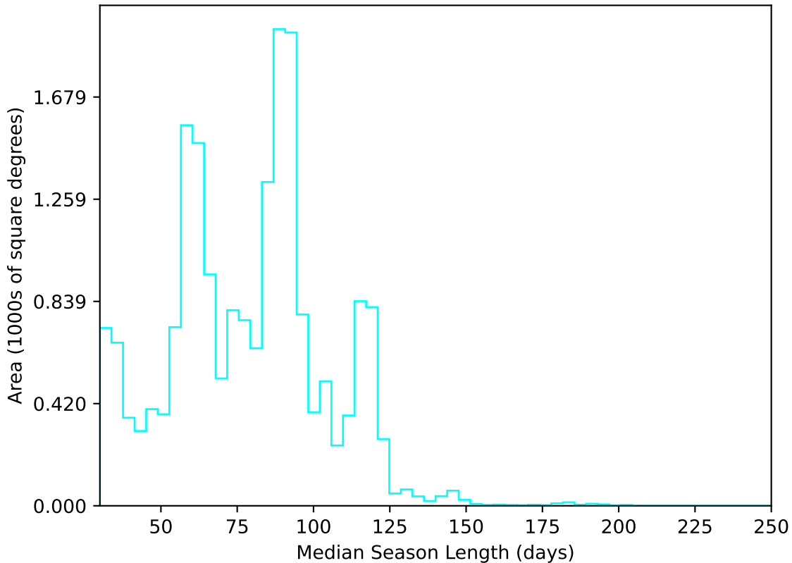
too_elab_r256_d2_griz_v3.4_10yrs All sky u band: Median Season Length
