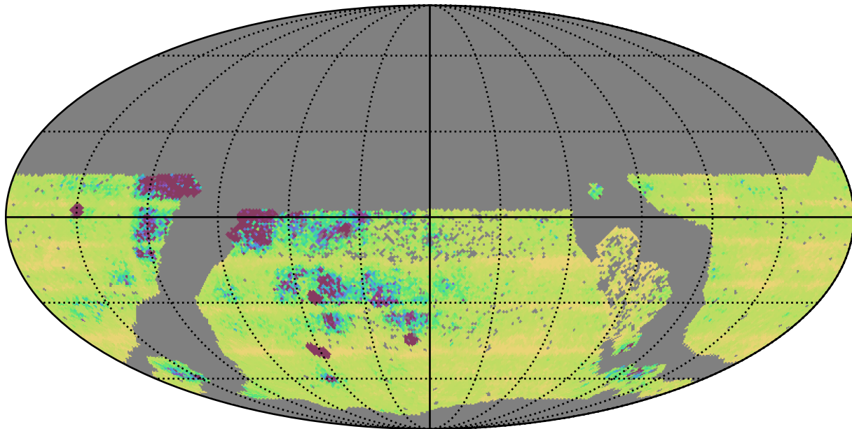
too_elab_r256_d2_griz_v3.4_10yrs WFD: Median Intra-Night Gap
