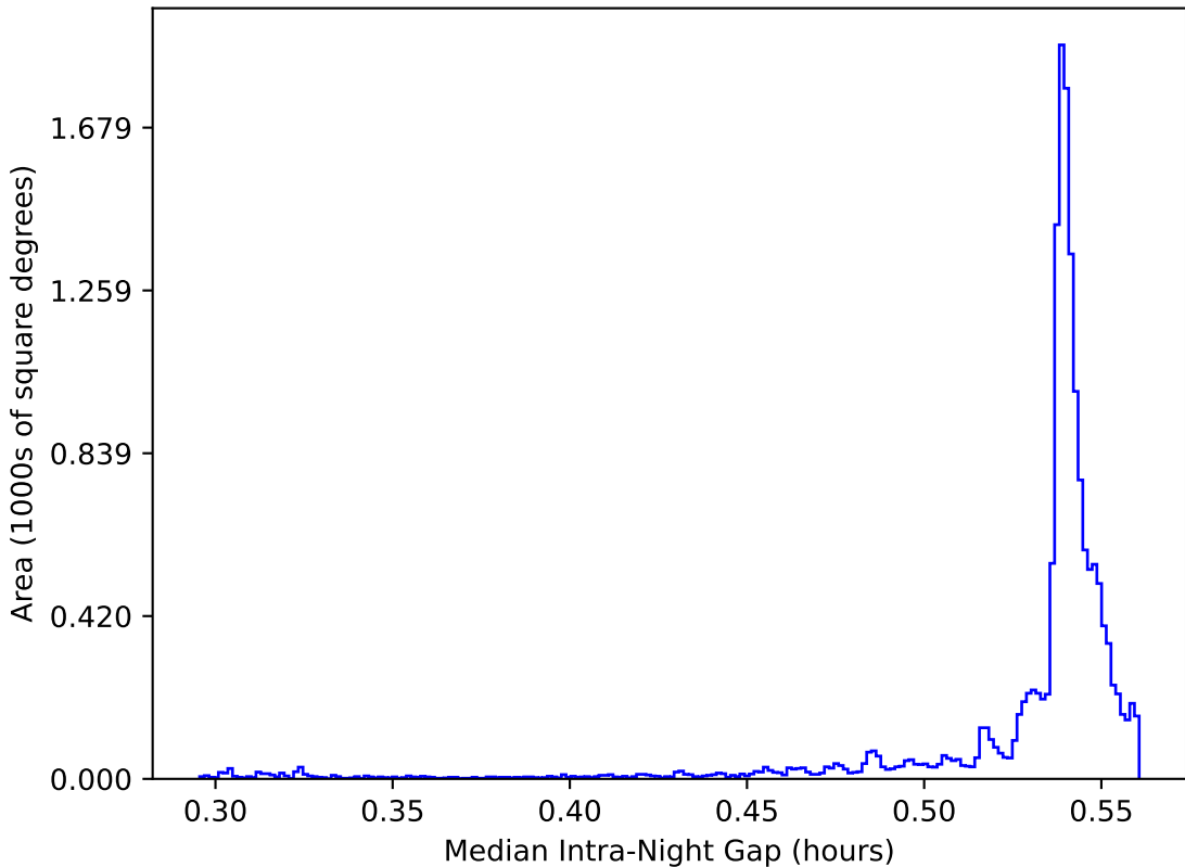
too_elab_r256_d2_griz_v3.4_10yrs WFD: Median Intra-Night Gap
