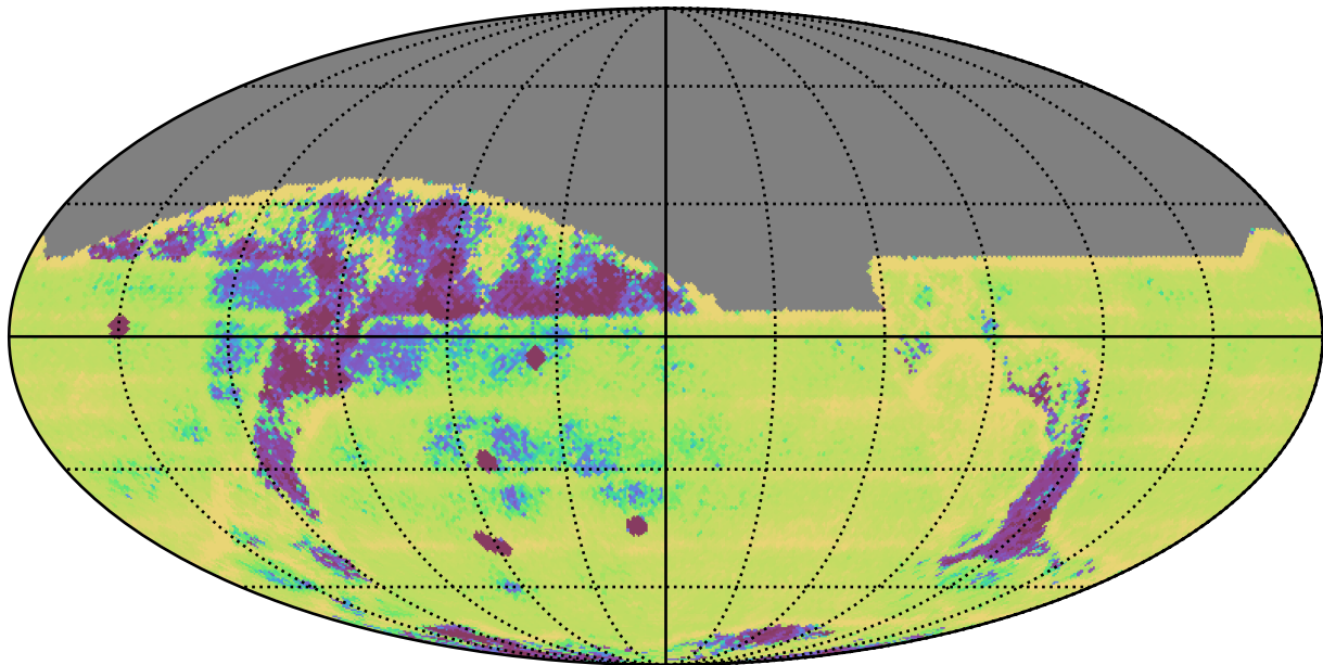
too_elab_r256_d2_griz_v3.4_10yrs All sky: Median Intra-Night Gap
