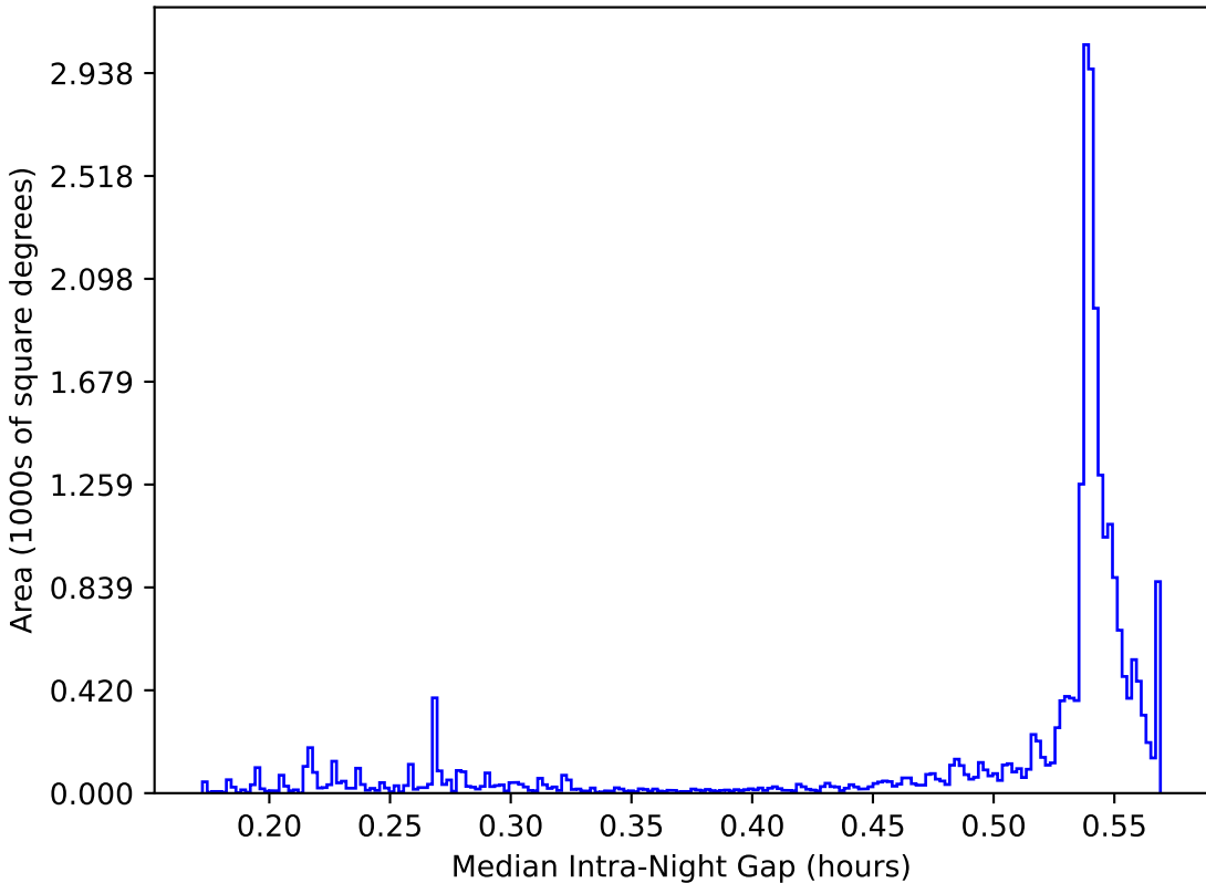
too_elab_r256_d2_griz_v3.4_10yrs All sky: Median Intra-Night Gap
