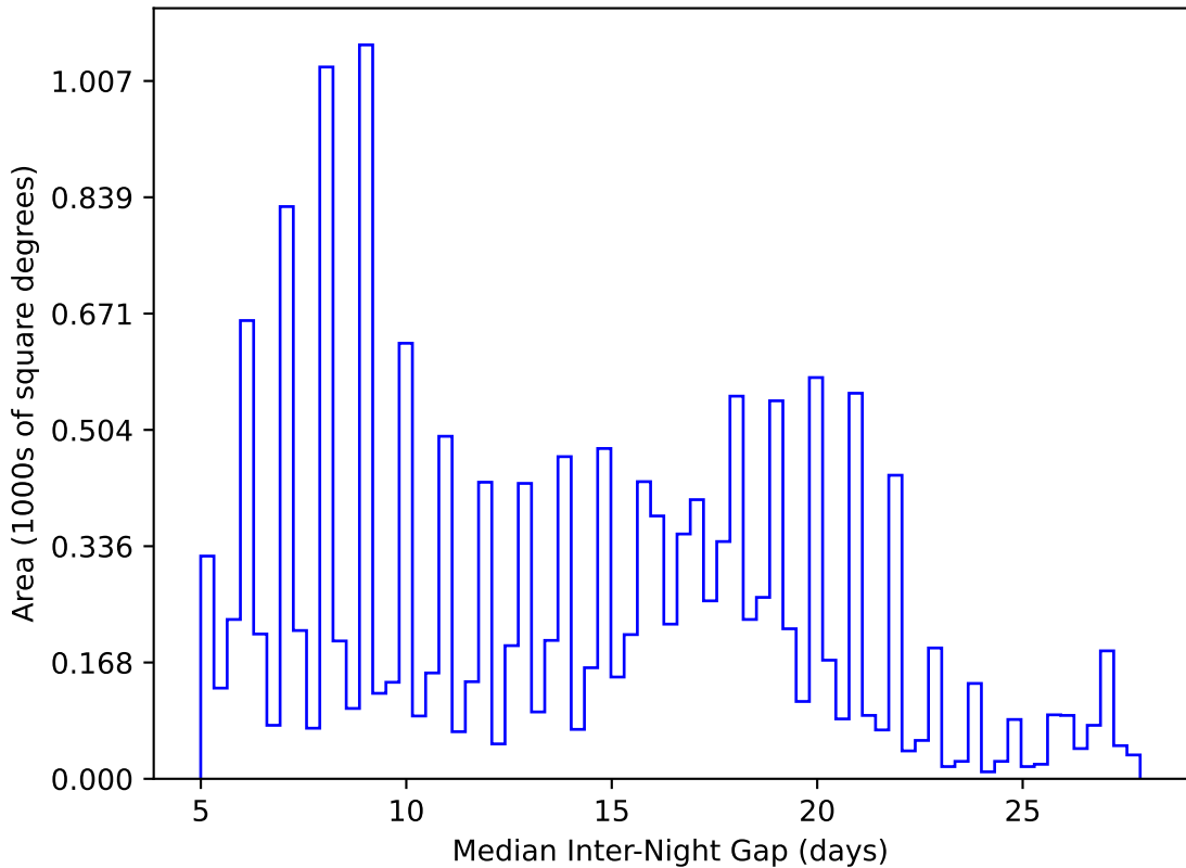
too_elab_r256_d2_griz_v3.4_10yrs WFD y band: Median Inter-Night Gap
