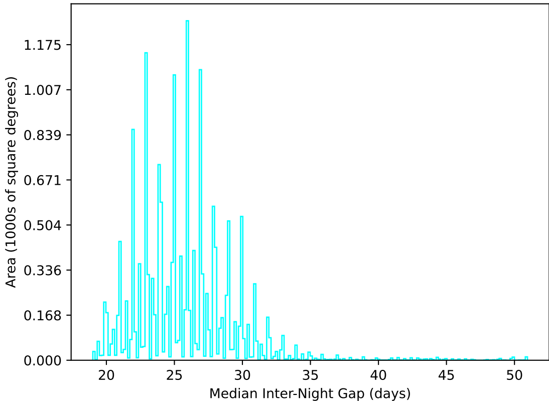
too_elab_r256_d2_griz_v3.4_10yrs WFD u band: Median Inter-Night Gap
