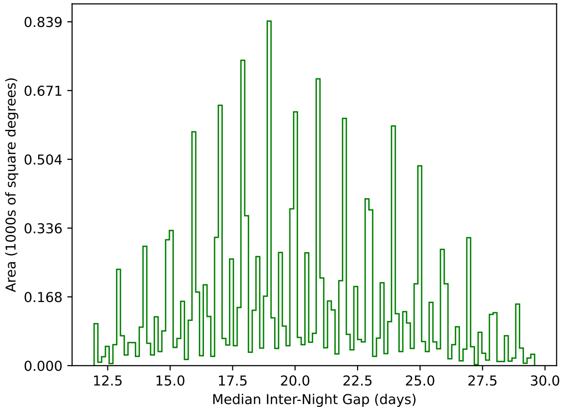
too_elab_r256_d2_griz_v3.4_10yrs WFD g band: Median Inter-Night Gap
