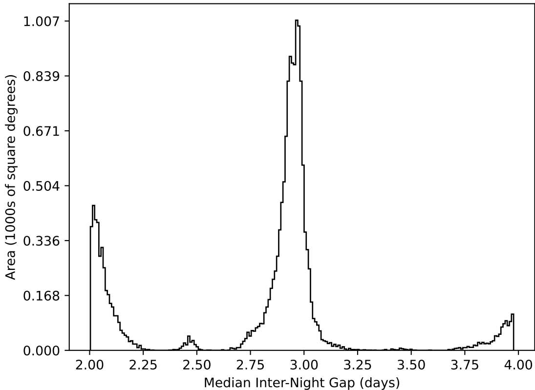
too_elab_r256_d2_griz_v3.4_10yrs WFD all bands: Median Inter-Night Gap
