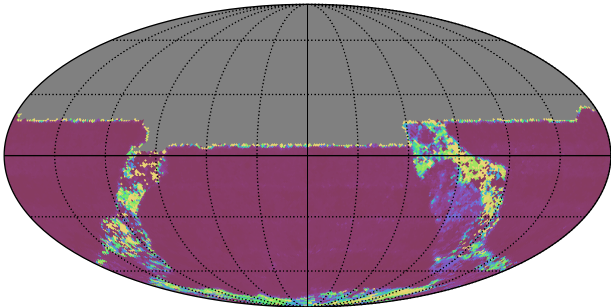
too_elab_r256_d2_griz_v3.4_10yrs All sky u band: Median Inter-Night Gap
