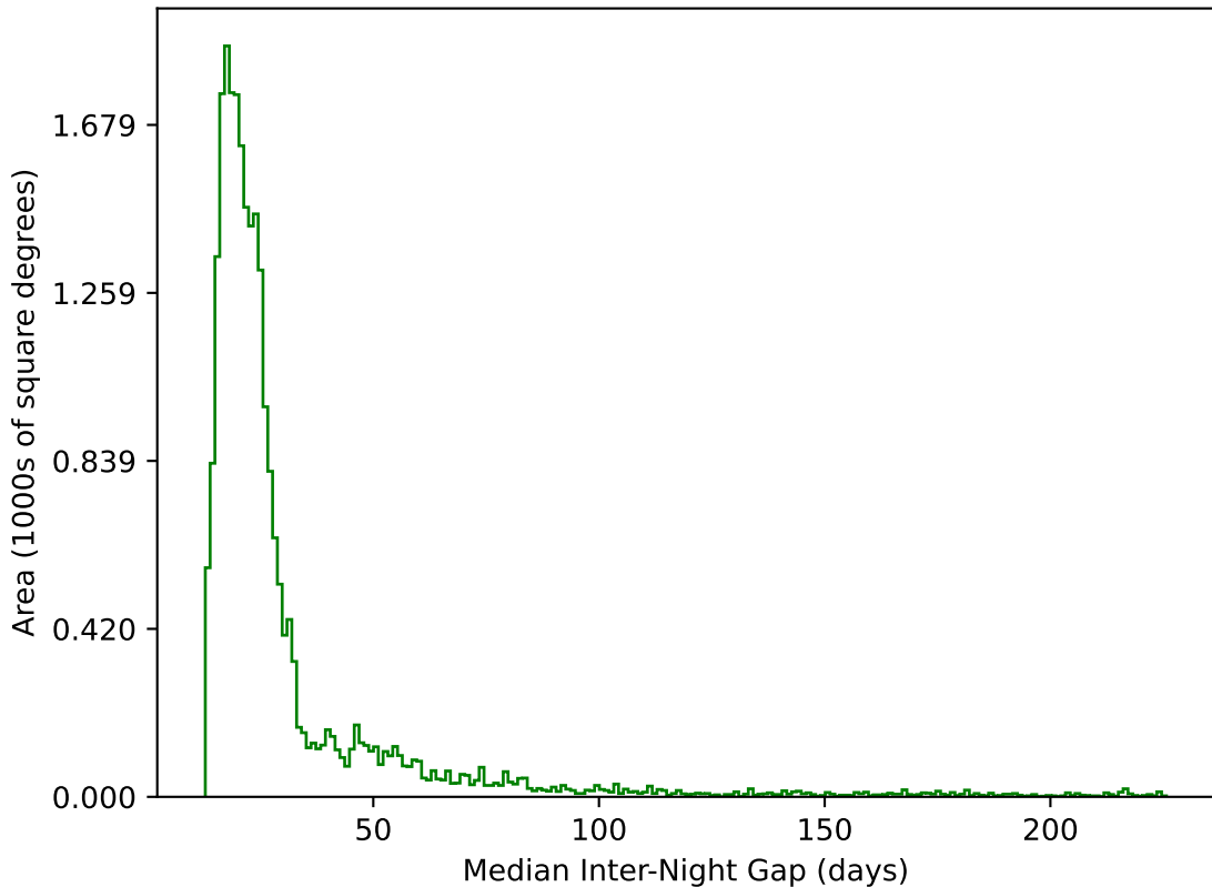
too_elab_r256_d2_griz_v3.4_10yrs All sky g band: Median Inter-Night Gap
