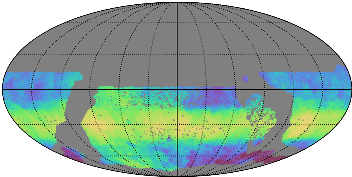
too_elab_r256_d2_griz_v3.4_10yrs WFD z band: Median HA
