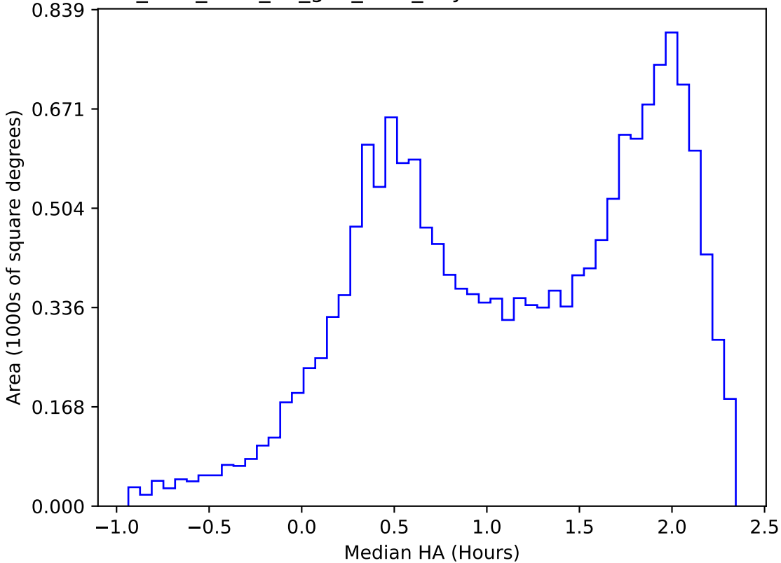
too_elab_r256_d2_griz_v3.4_10yrs WFD z band: Median HA
