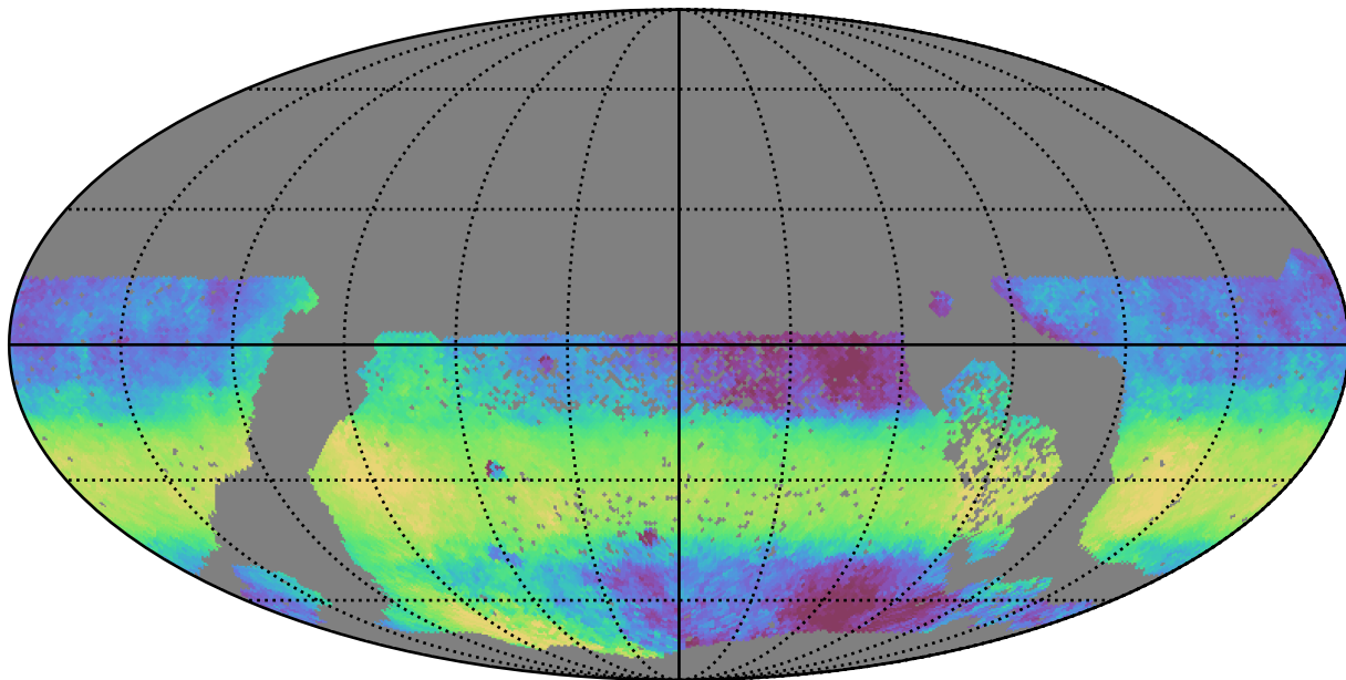
too_elab_r256_d2_griz_v3.4_10yrs WFD y band: Median HA
