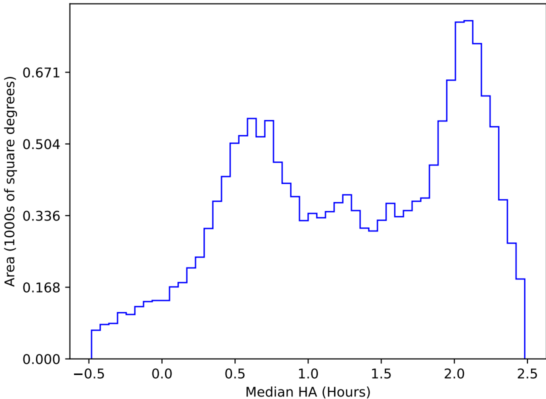
too_elab_r256_d2_griz_v3.4_10yrs WFD y band: Median HA
