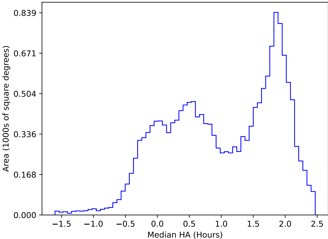
too_elab_r256_d2_griz_v3.4_10yrs WFD u band: Median HA
