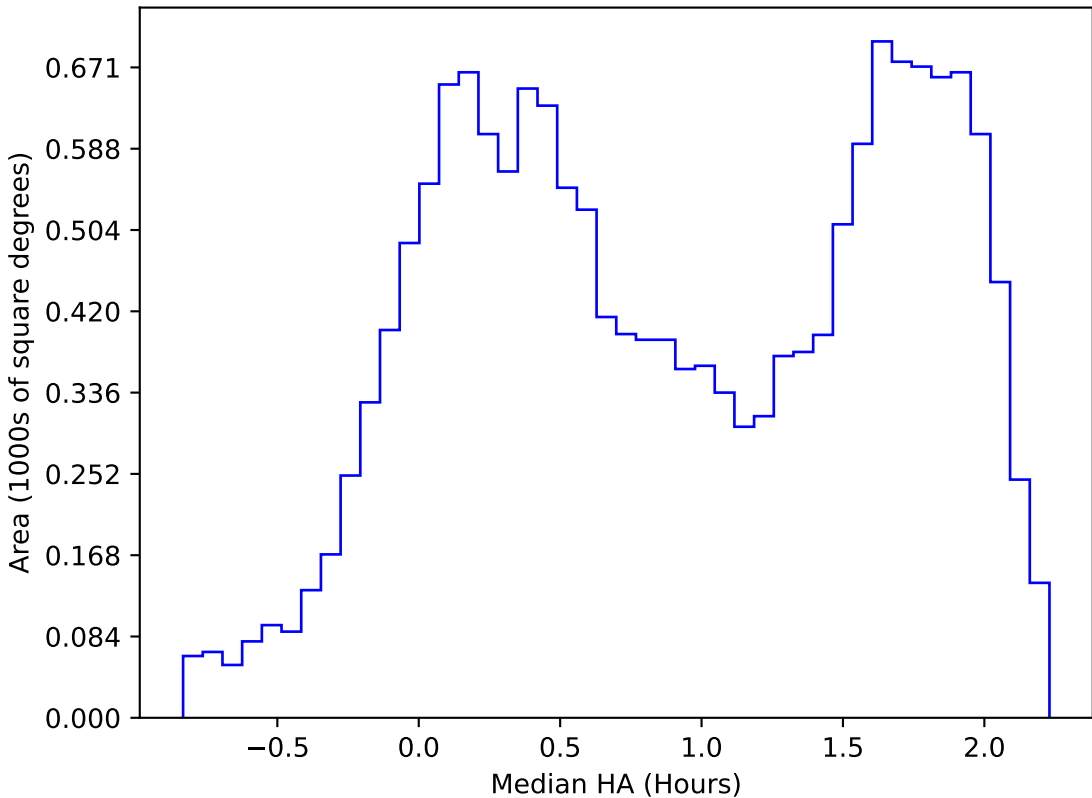
too_elab_r256_d2_griz_v3.4_10yrs WFD r band: Median HA
