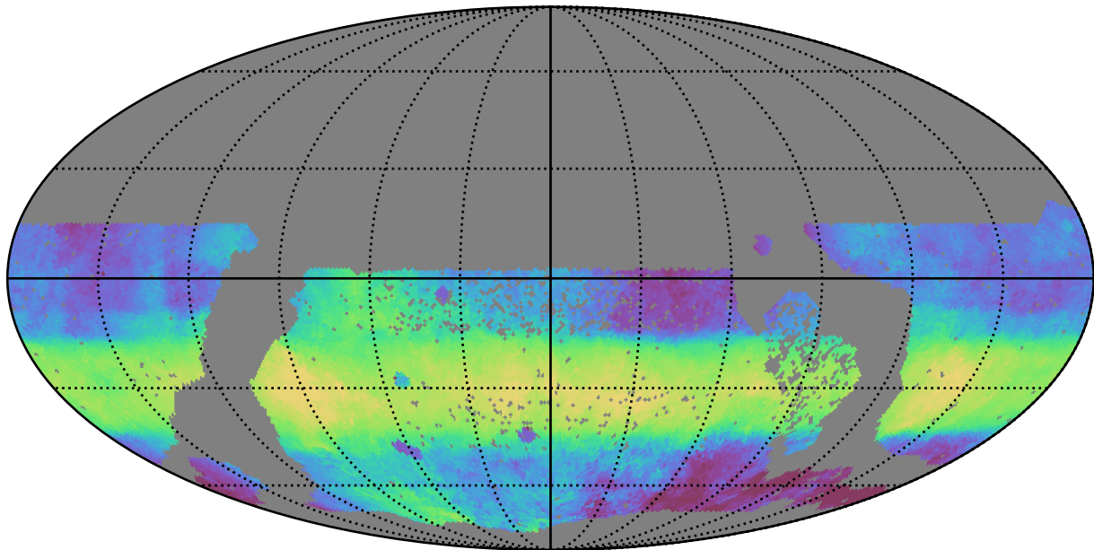
too_elab_r256_d2_griz_v3.4_10yrs WFD i band: Median HA
