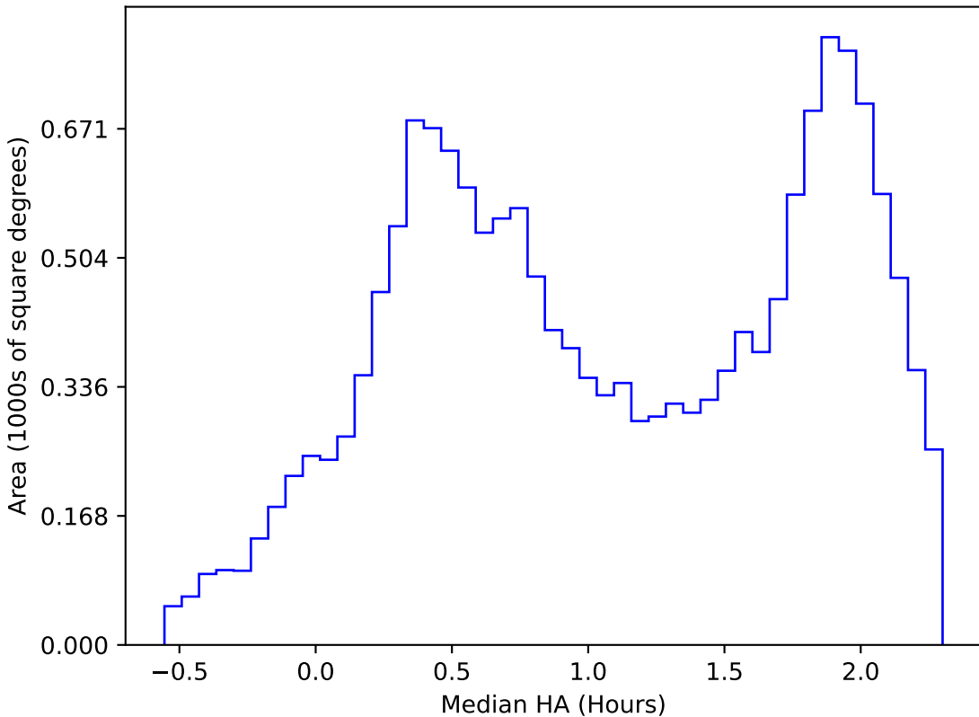
too_elab_r256_d2_griz_v3.4_10yrs WFD i band: Median HA
