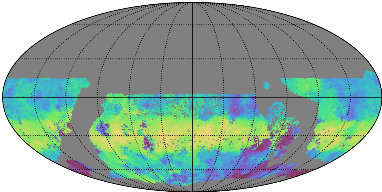
too_elab_r256_d2_griz_v3.4_10yrs WFD g band: Median HA
