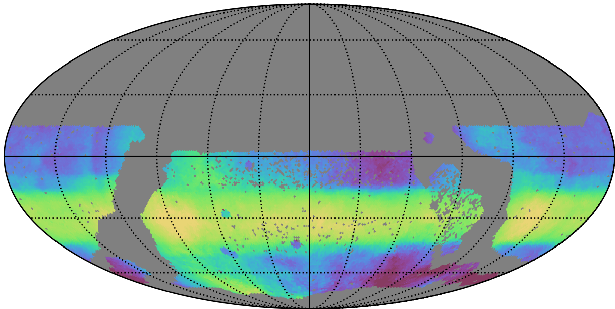
too_elab_r256_d2_griz_v3.4_10yrs WFD all bands: Median HA
