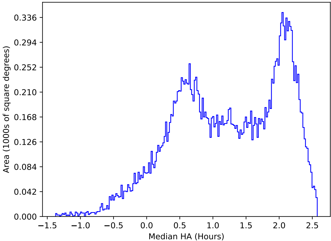
too_elab_r256_d2_griz_v3.4_10yrs All sky y band: Median HA
