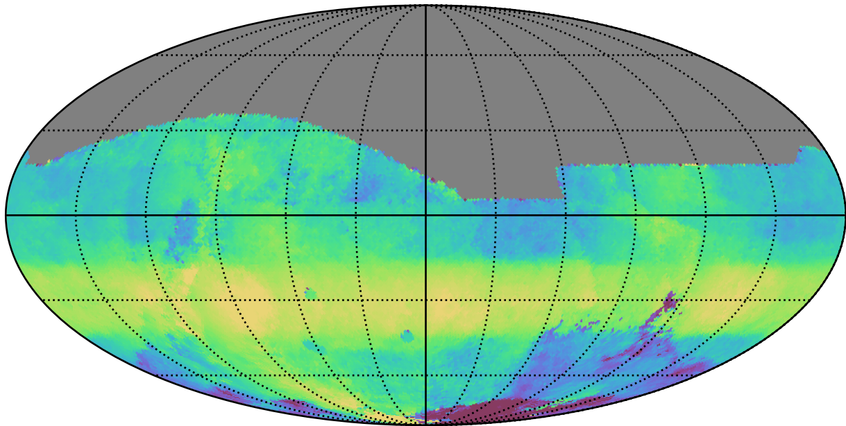
too_elab_r256_d2_griz_v3.4_10yrs All sky r band: Median HA
