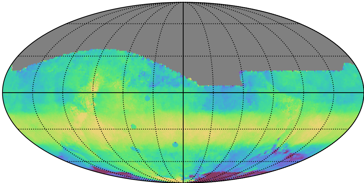
too_elab_r256_d2_griz_v3.4_10yrs All sky i band: Median HA
