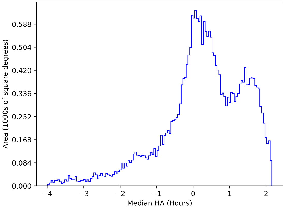
too_elab_r256_d2_griz_v3.4_10yrs All sky g band: Median HA
