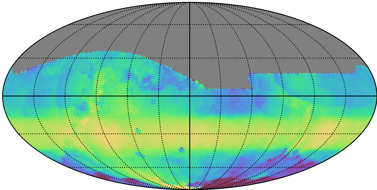
too_elab_r256_d2_griz_v3.4_10yrs All sky all bands: Median HA
