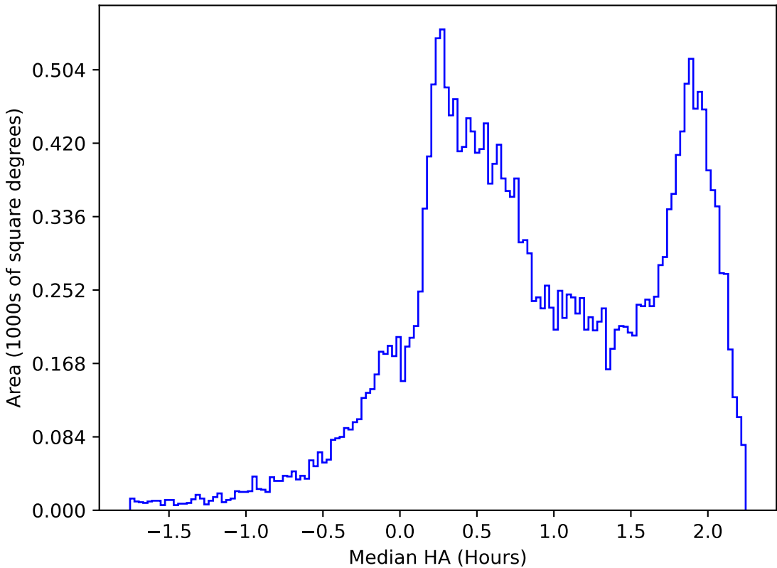
too_elab_r256_d2_griz_v3.4_10yrs All sky all bands: Median HA
