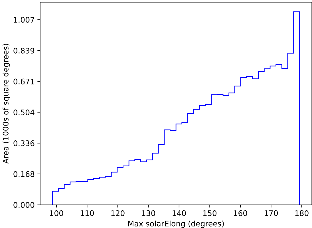
too_elab_r256_d2_griz_v3.4_10yrs WFD z band: Max solarElong
