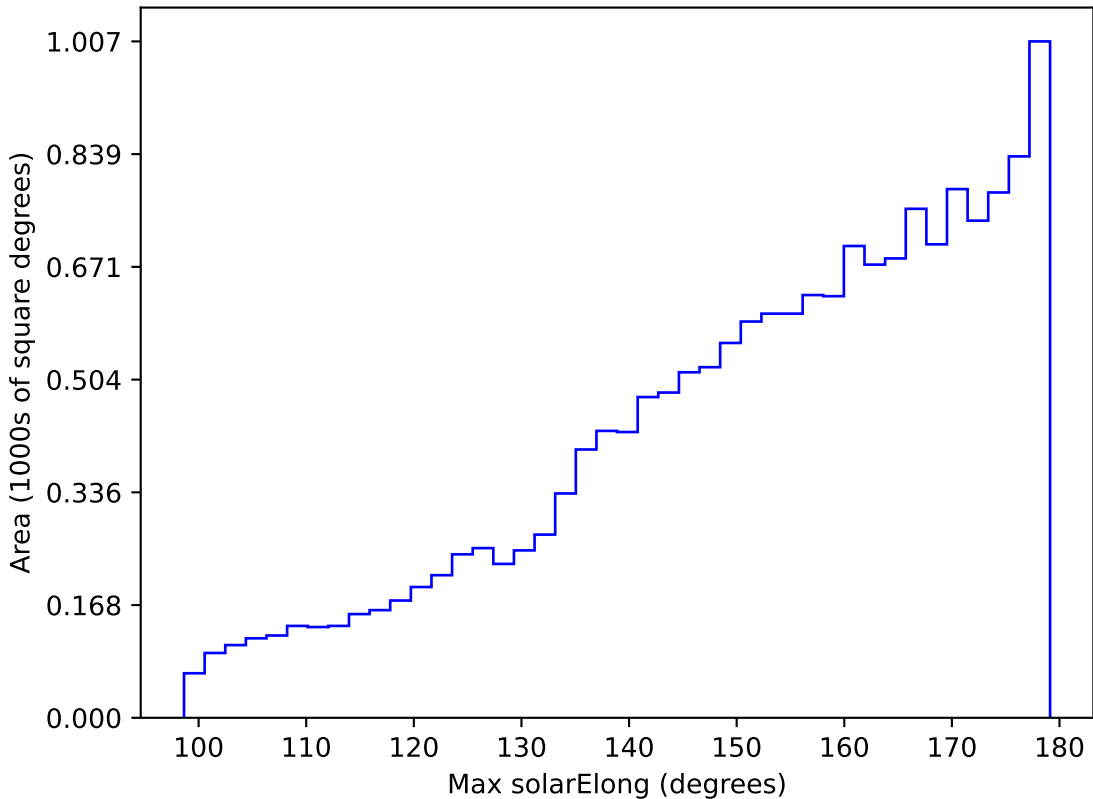
too_elab_r256_d2_griz_v3.4_10yrs WFD y band: Max solarElong
