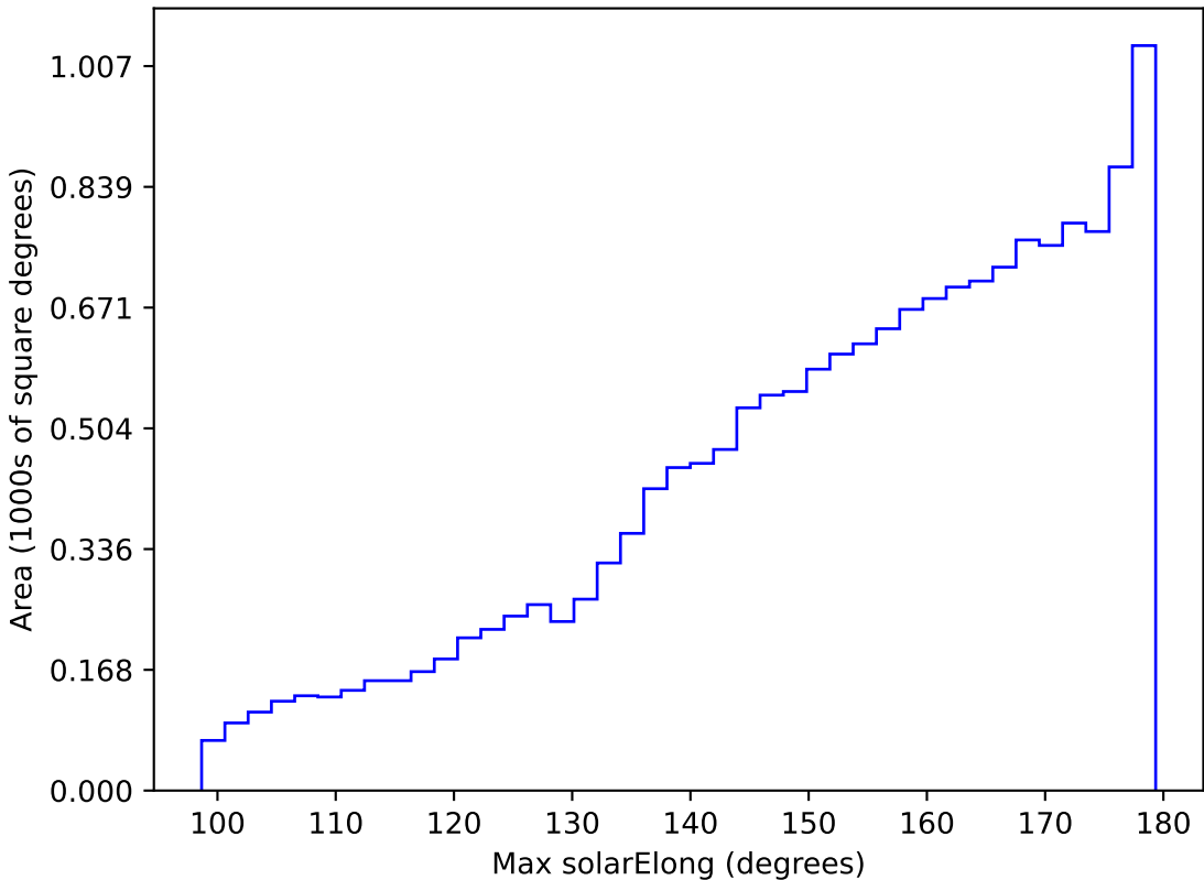
too_elab_r256_d2_griz_v3.4_10yrs WFD i band: Max solarElong
