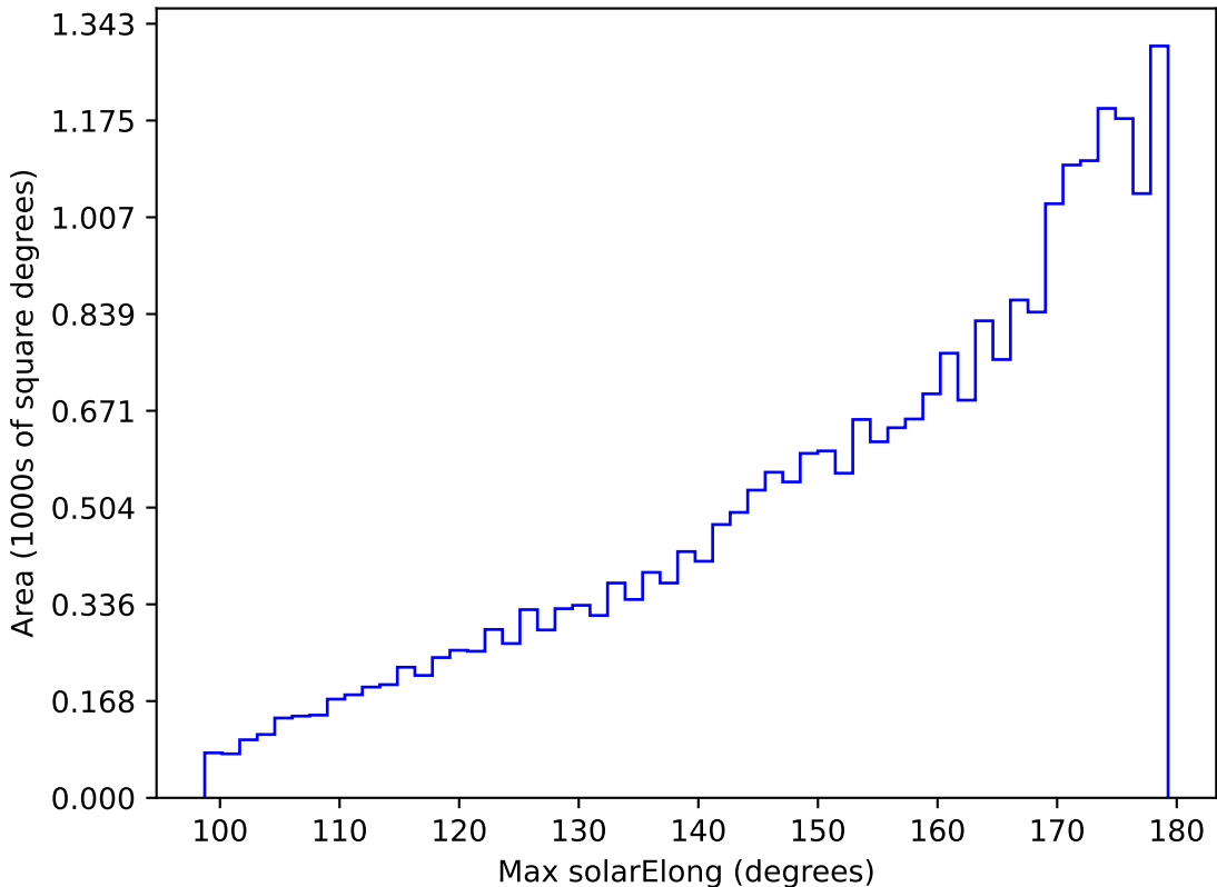
too_elab_r256_d2_griz_v3.4_10yrs All sky z band: Max solarElong
