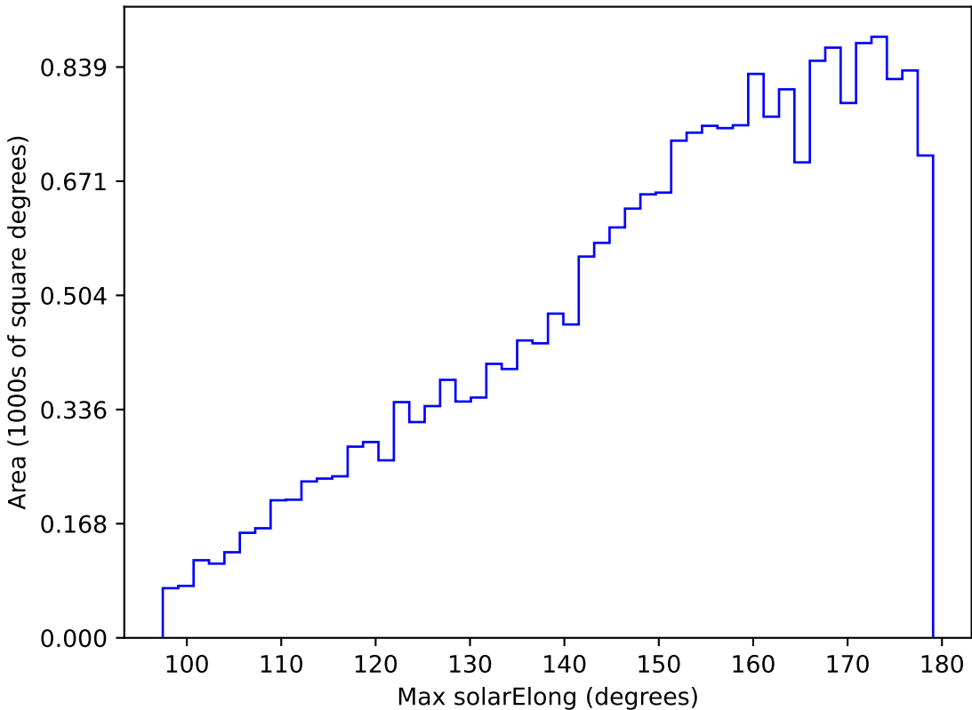
too_elab_r256_d2_griz_v3.4_10yrs All sky u band: Max solarElong
