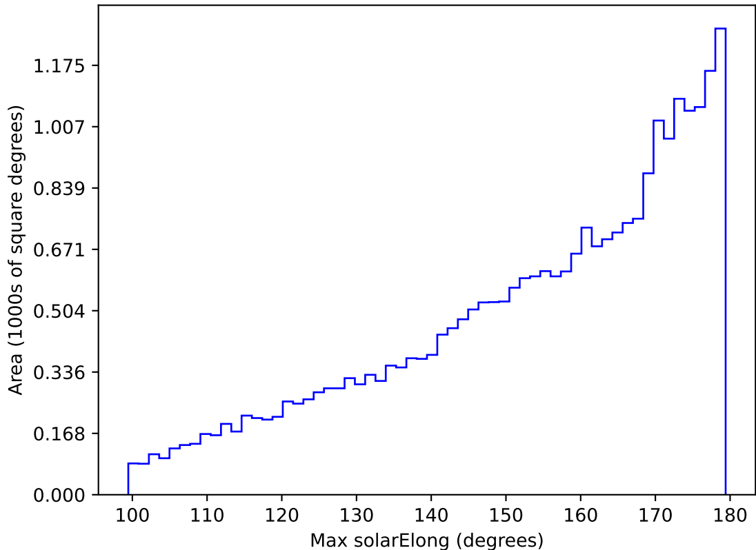
too_elab_r256_d2_griz_v3.4_10yrs All sky i band: Max solarElong
