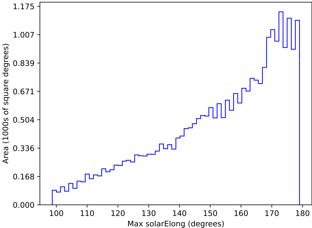
too_elab_r256_d2_griz_v3.4_10yrs All sky g band: Max solarElong
