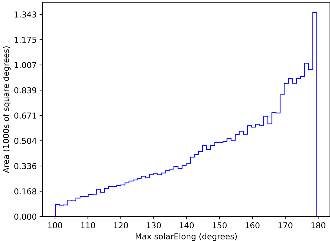
too_elab_r256_d2_griz_v3.4_10yrs All sky all bands: Max solarElong
