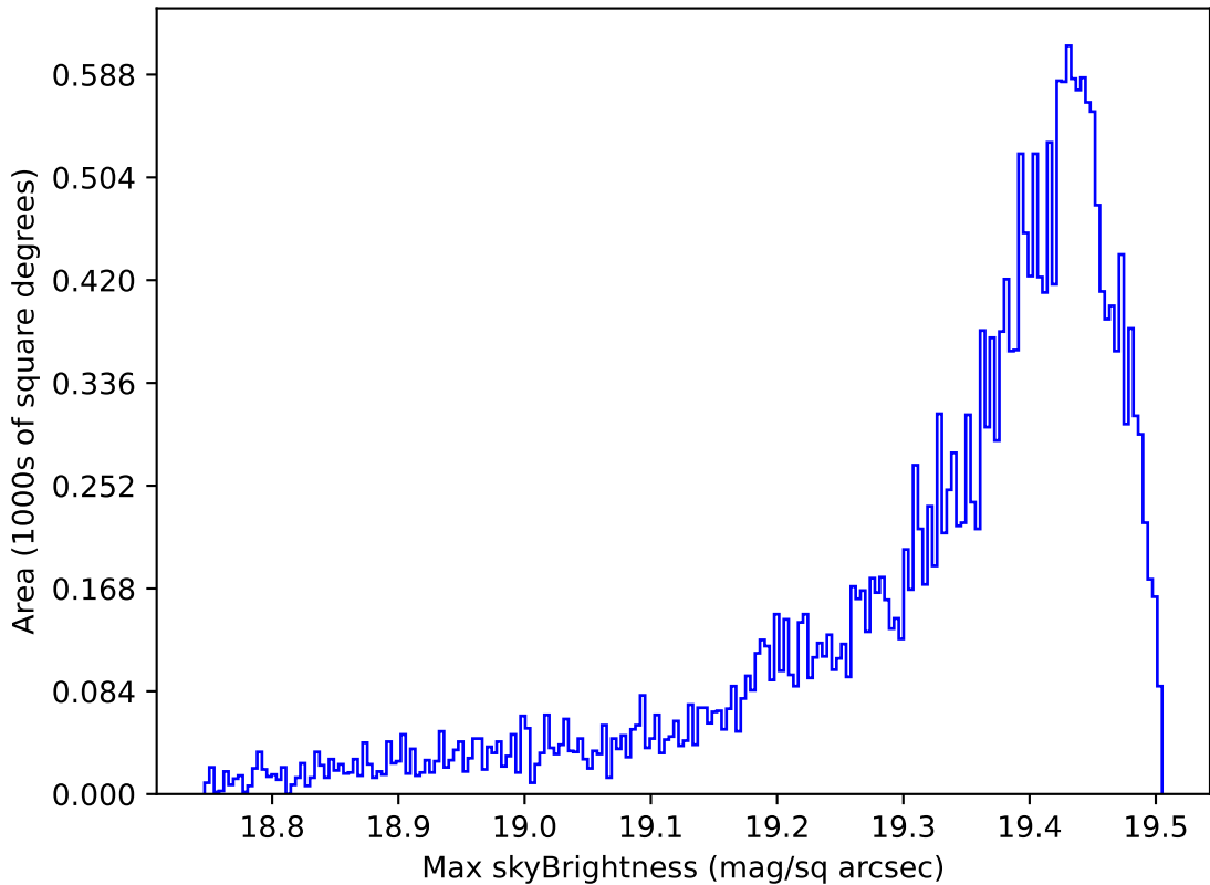
too_elab_r256_d2_griz_v3.4_10yrs Yr 1 z band: Max skyBrightness
