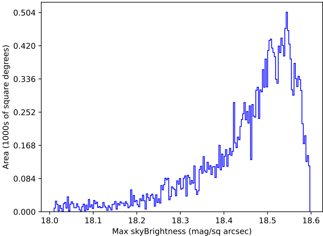
too_elab_r256_d2_griz_v3.4_10yrs Yr 1 y band: Max skyBrightness
