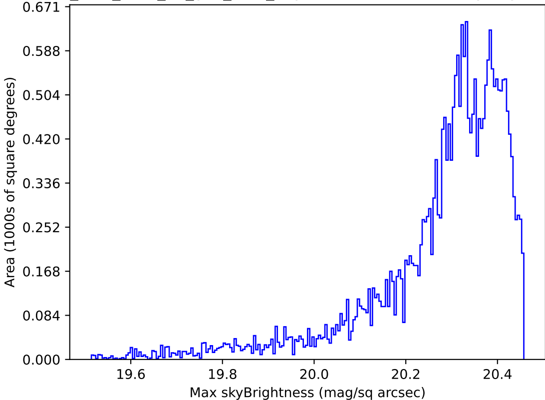
too_elab_r256_d2_griz_v3.4_10yrs Yr 1 i band: Max skyBrightness
