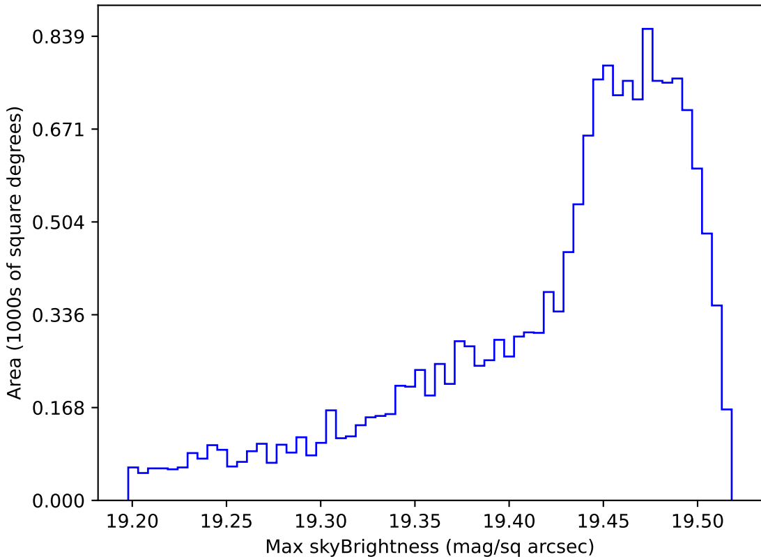
too_elab_r256_d2_griz_v3.4_10yrs WFD z band: Max skyBrightness
