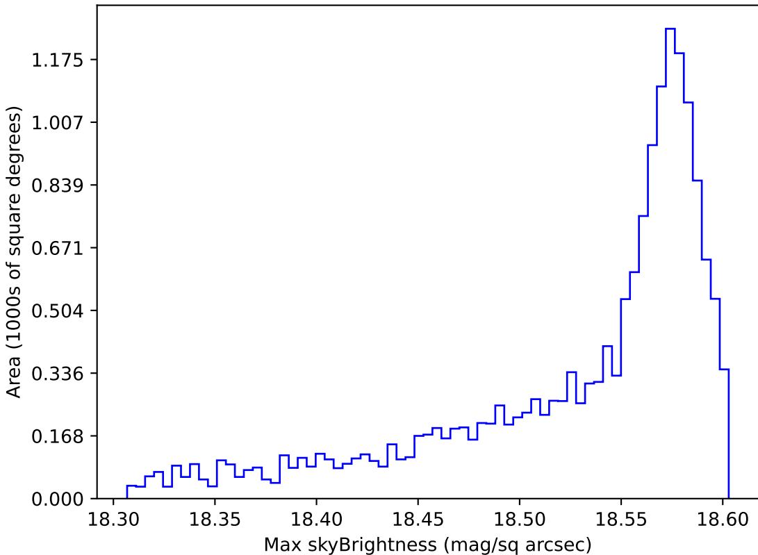
too_elab_r256_d2_griz_v3.4_10yrs WFD y band: Max skyBrightness
