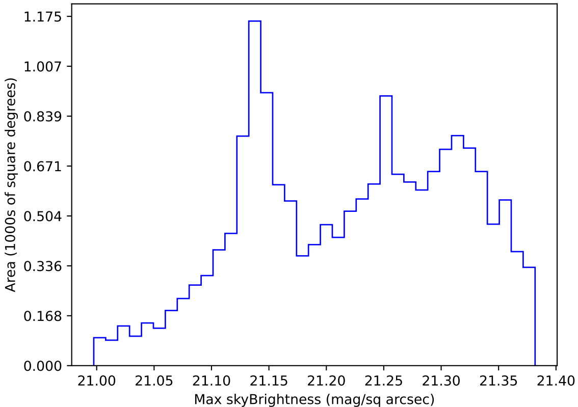
too_elab_r256_d2_griz_v3.4_10yrs WFD r band: Max skyBrightness
