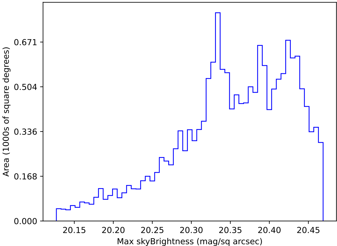
too_elab_r256_d2_griz_v3.4_10yrs WFD i band: Max skyBrightness
