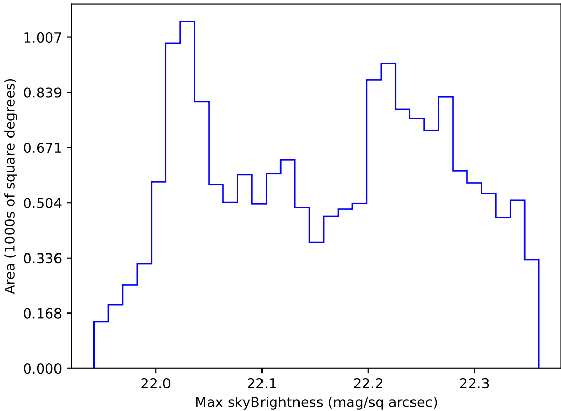
too_elab_r256_d2_griz_v3.4_10yrs WFD g band: Max skyBrightness
