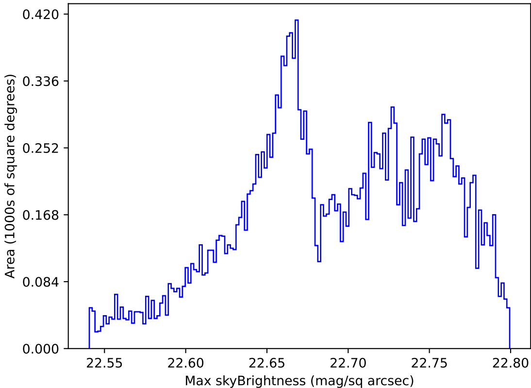
too_elab_r256_d2_griz_v3.4_10yrs All sky u band: Max skyBrightness
