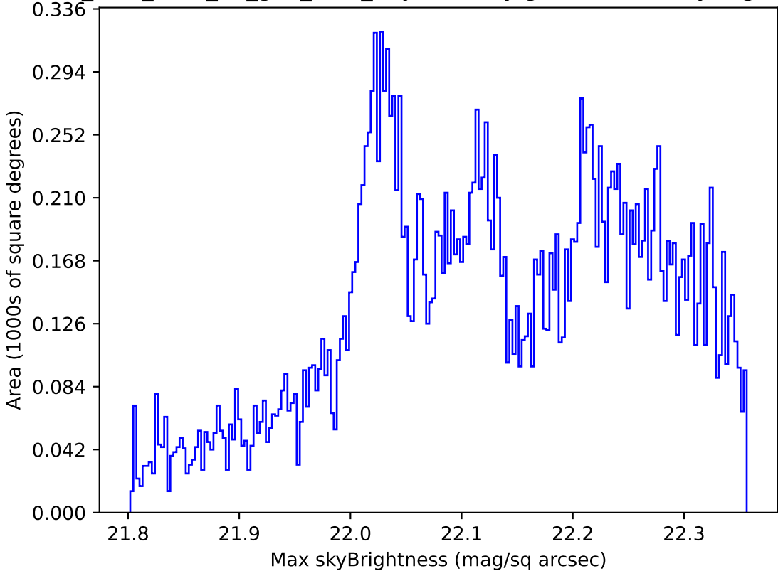
too_elab_r256_d2_griz_v3.4_10yrs All sky g band: Max skyBrightness
