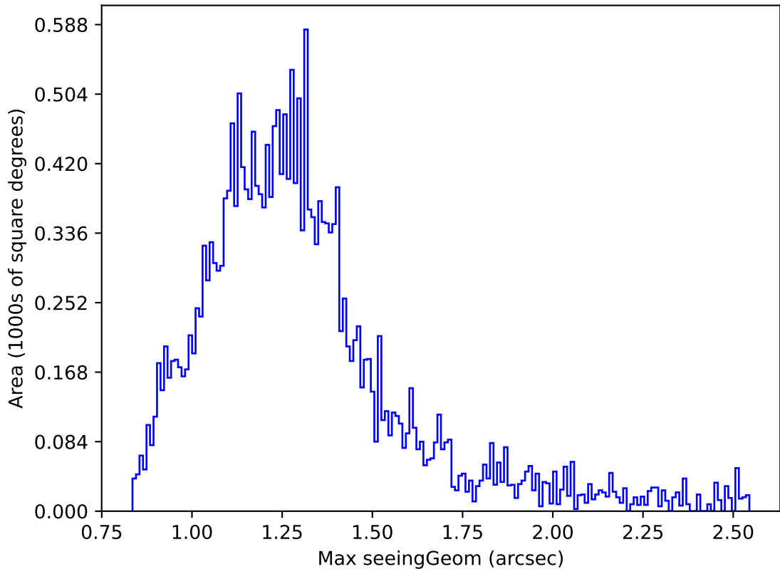
too_elab_r256_d2_griz_v3.4_10yrs Yr 1 y band: Max seeingGeom
