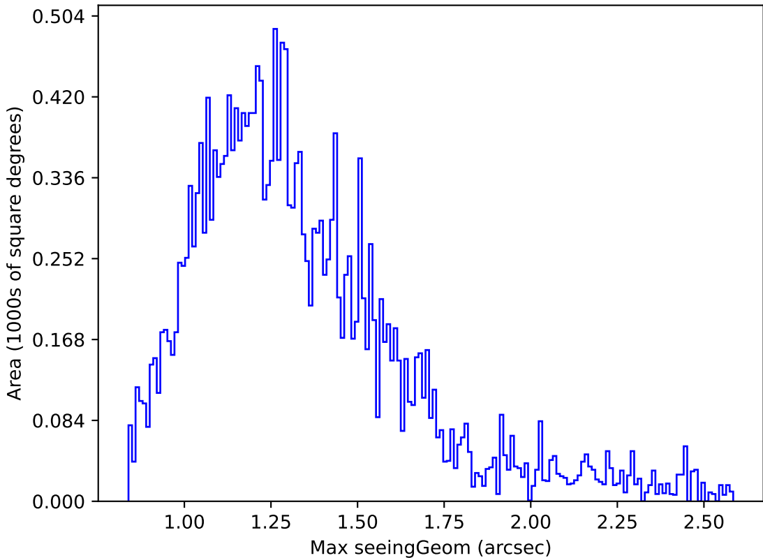
too_elab_r256_d2_griz_v3.4_10yrs Yr 1 u band: Max seeingGeom
