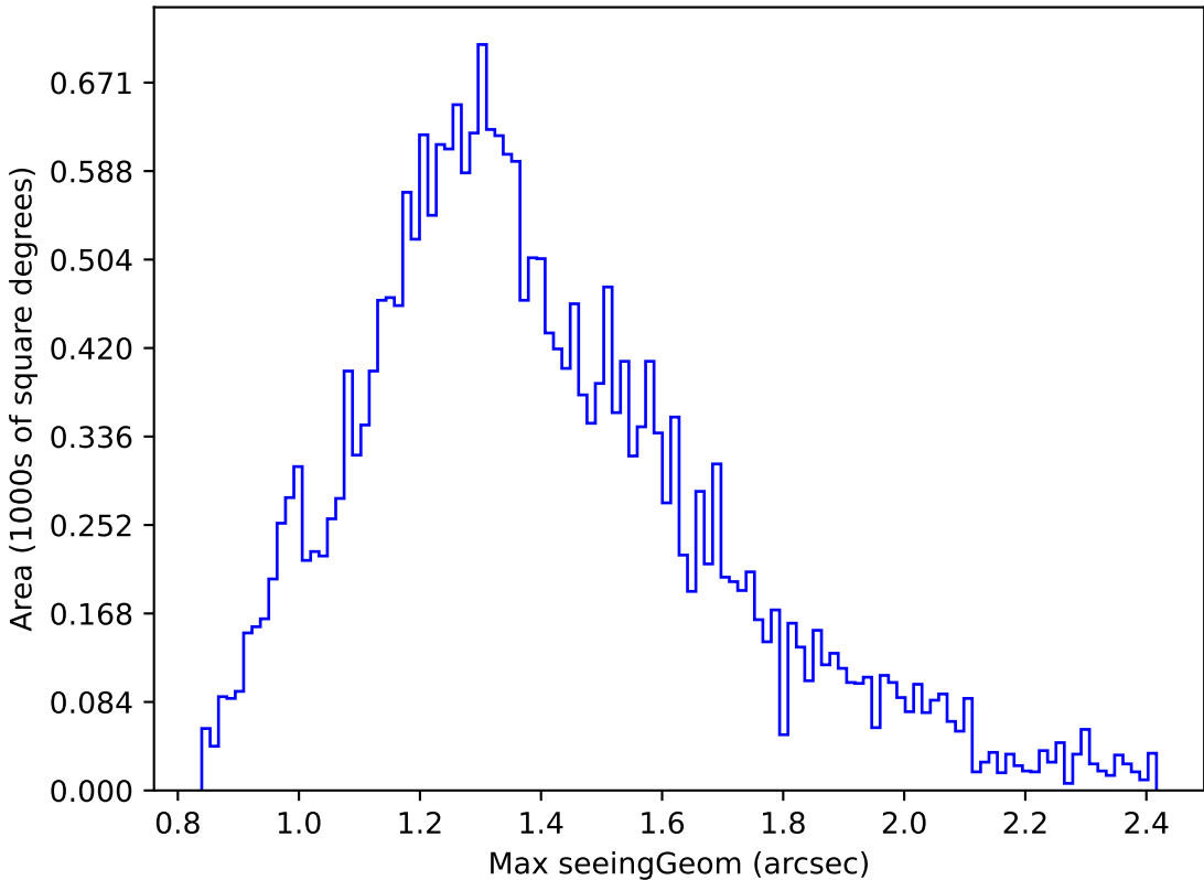
too_elab_r256_d2_griz_v3.4_10yrs Yr 1 r band: Max seeingGeom
