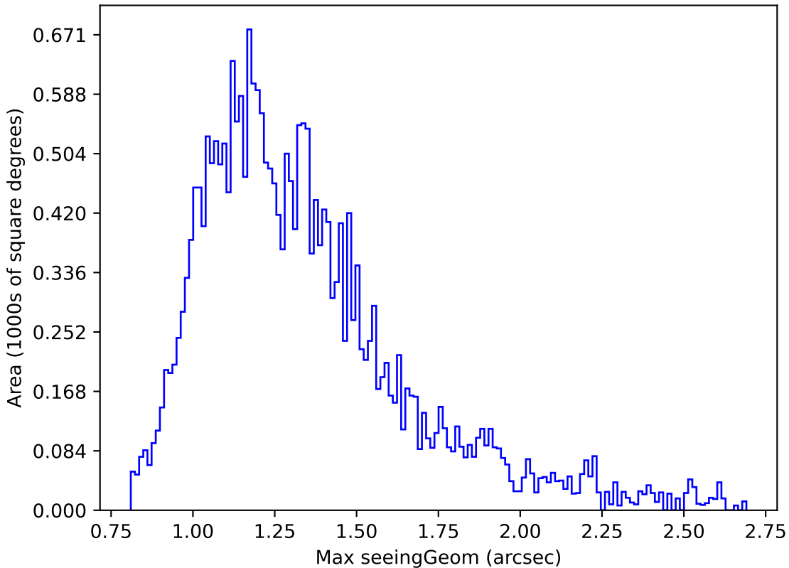
too_elab_r256_d2_griz_v3.4_10yrs Yr 1 i band: Max seeingGeom
