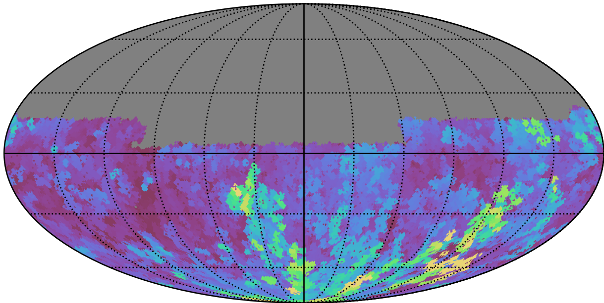
too_elab_r256_d2_griz_v3.4_10yrs Yr 1 u band: Max seeingEff
